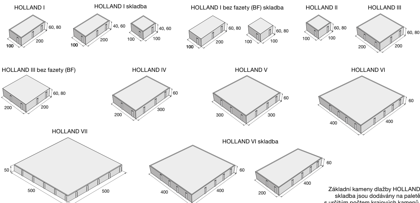
HOLLAND – colormix Piano
