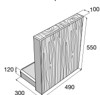
STANDARD S 55/R, reliéf – prkno
